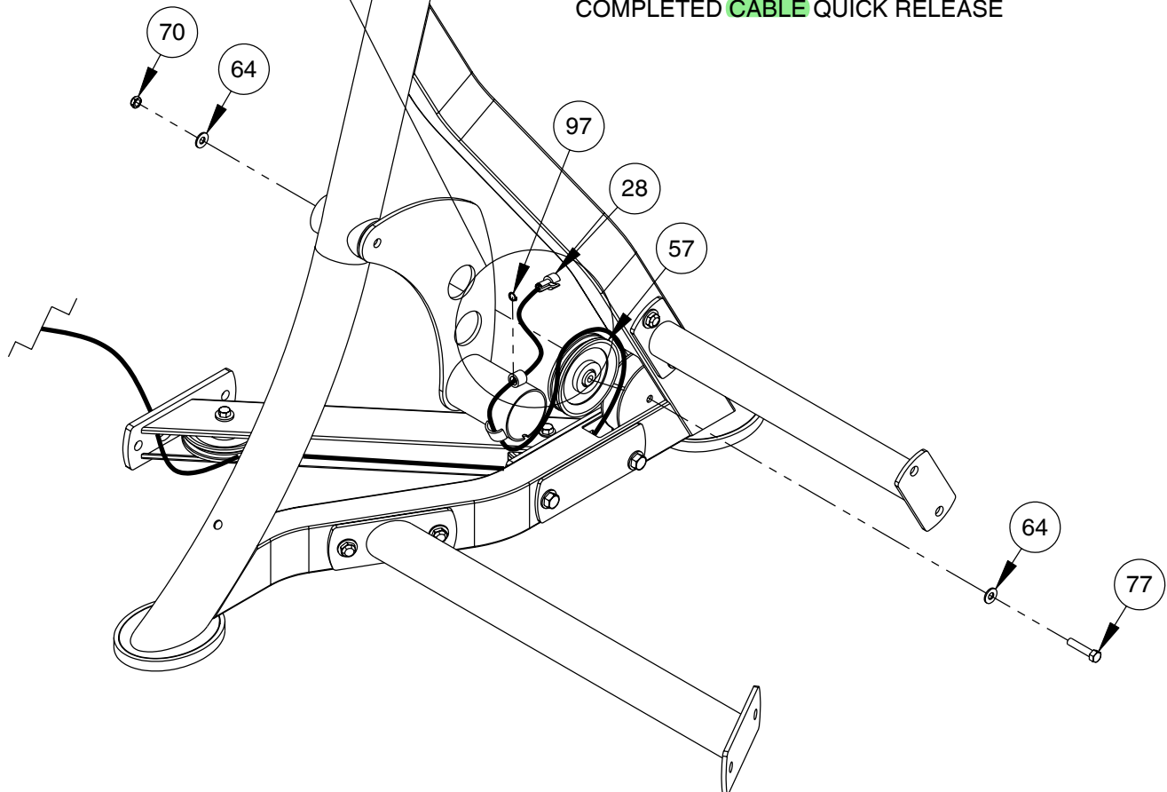
DETAIL VIEW COMPLETED CABLE QUICK RELEASE
