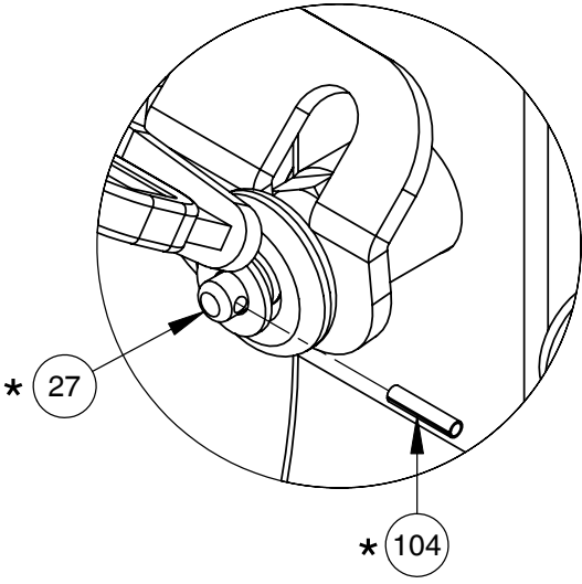
DETAIL B SCALE 1 : 1.5
