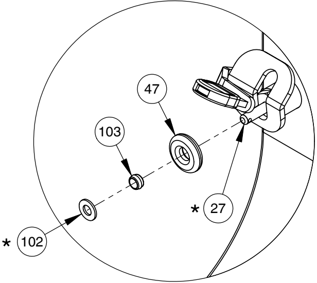
DETAIL A SCALE 1 : 3
